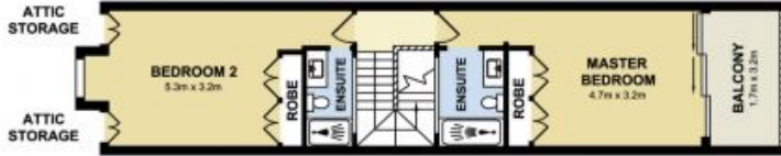
FIRST FLOOR
