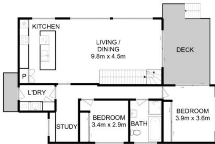
UPPER FLOOR
