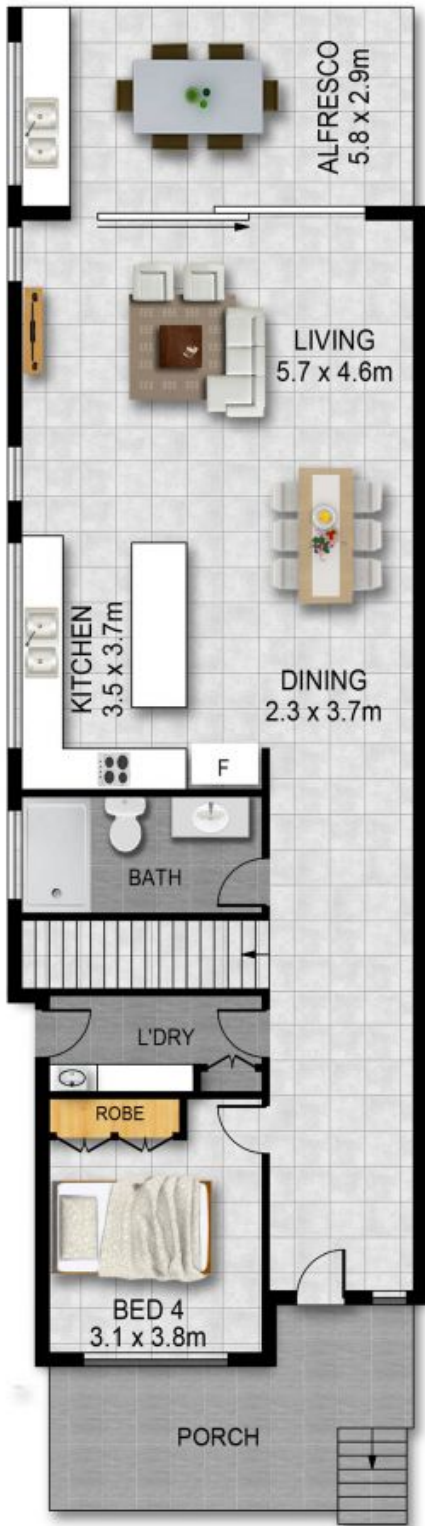
GROUND FLOOR
