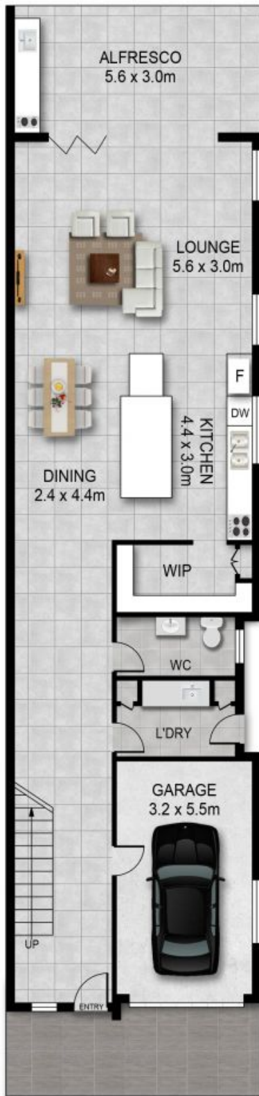
GROUND FLOOR
