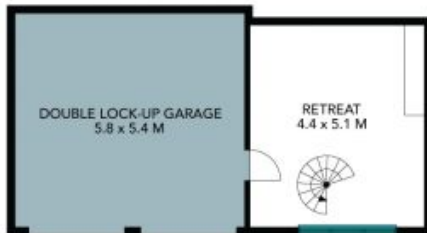
Lower Level
