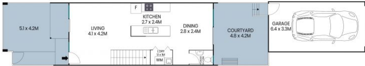
Ground Floor
