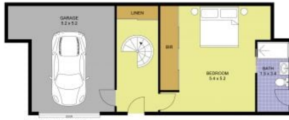
GROUND FLOOR
