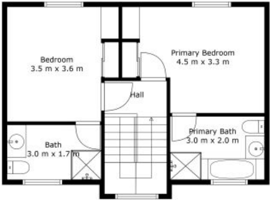
Floor 2
