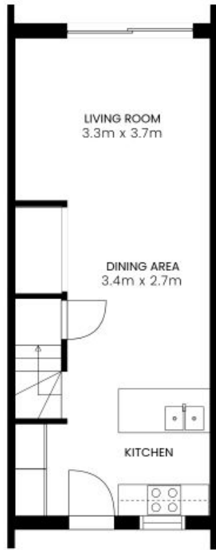
FLOOR 1
