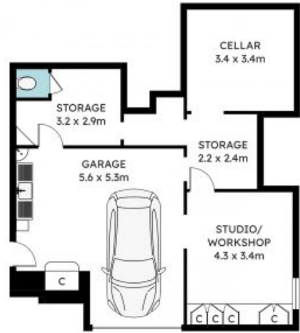
LOWER FLOOR
