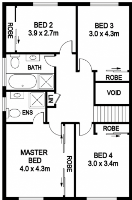
UPPER FLOOR
