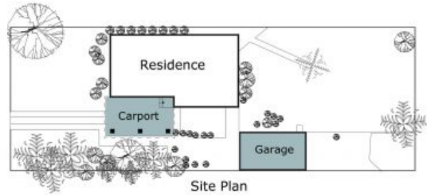
Site Plan
