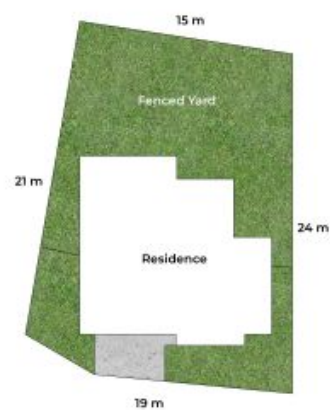
Site Plan
