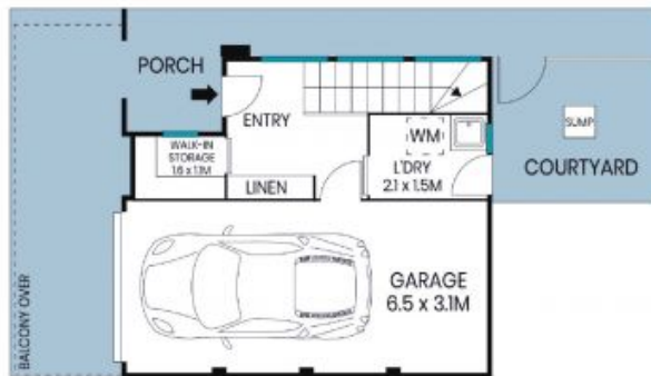
Lower Level (Unit 2)
