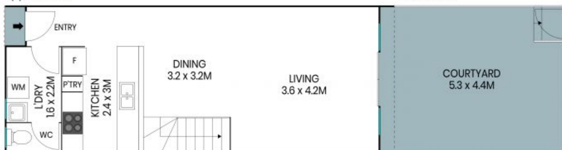
Ground Level
